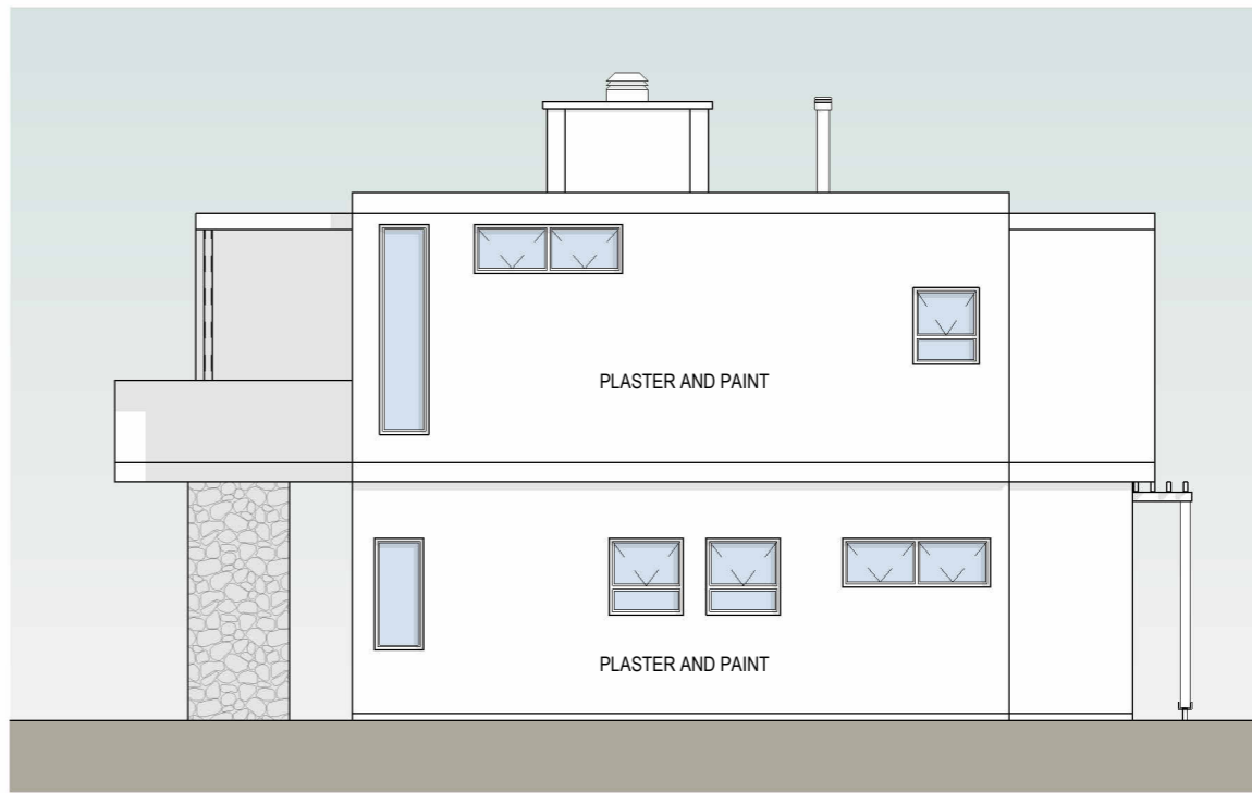
ELEVATION EAST
