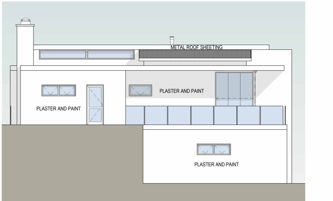
ELEVATION WEST
