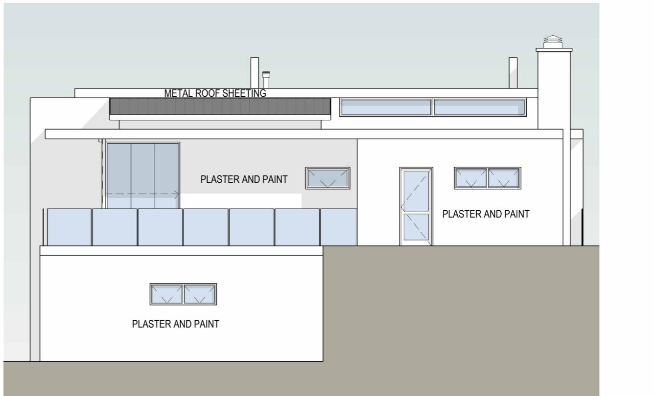
ELEVATION EAST
