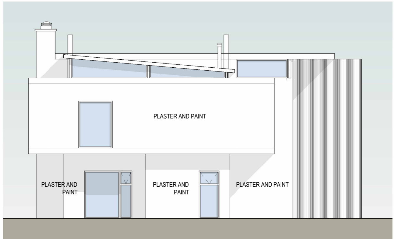
ELEVATION WEST
